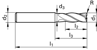
Series 3891 / 3892 - 3-flute end mill Standard length with neck clearance (Metric)
